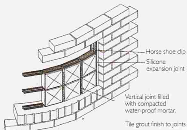
Standard construction curved Blokup glass block wall
